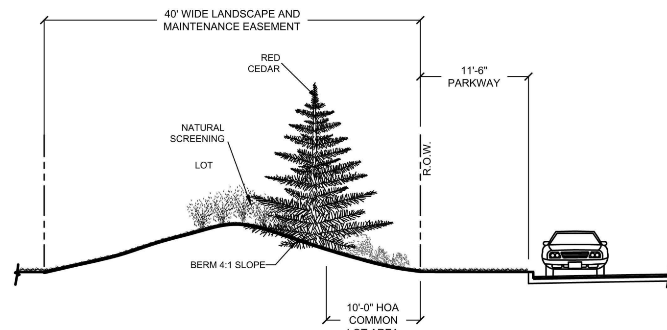
LANDSCAPE BUFFER ELEVATION
