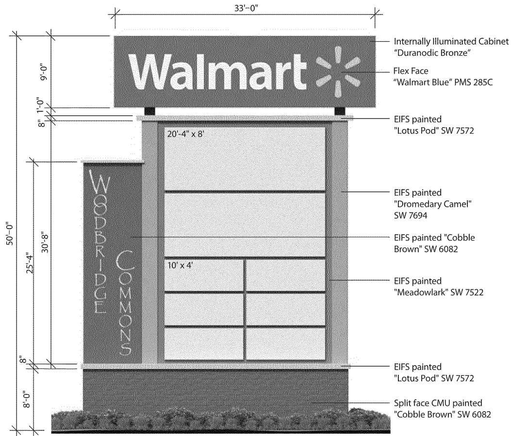
50' Pylon Sign Front Elevation Opt 1
