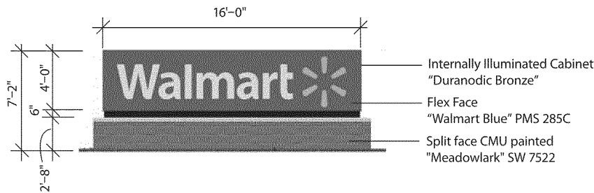
Monument Sign Front Elevation
